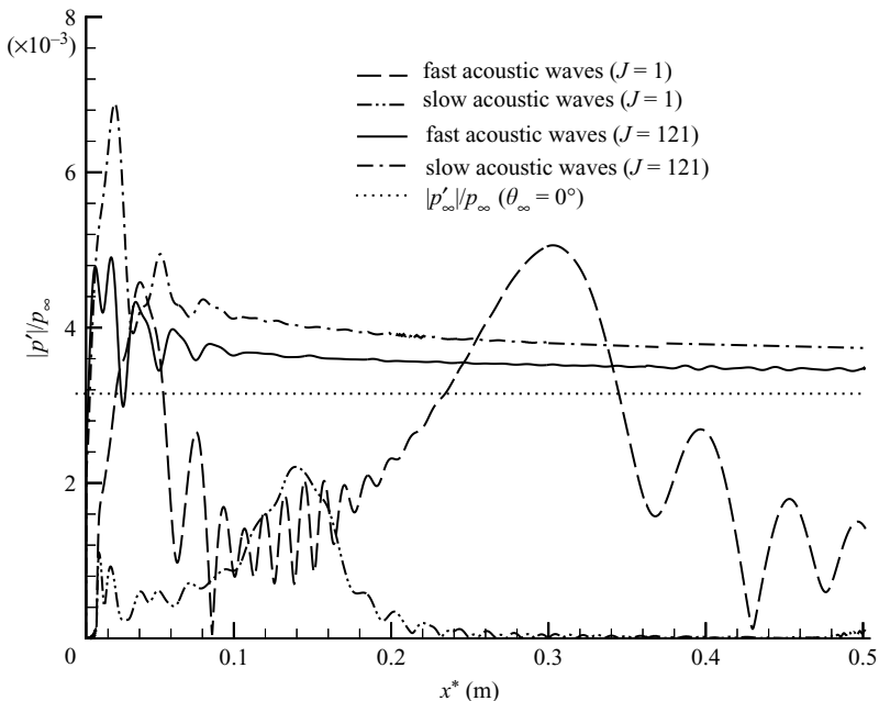
FIGURE 12. Distributions of pressure perturbation amplitudes induced by free-stream plane slow acoustic waves (case S.1). The results are compared with the corresponding results induced by free-stream fast acoustic waves (case F.1) ( M_\infty = 4.5 , F = 2.2 \times 10^{-4} and \theta_\infty = 0^\circ ).
