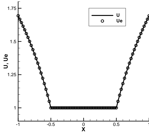
Fig. 13. Comparison of the profiles of the exact ( u_e ) and numerical ( u ) solutions along the horizontal center line. The numerical solution is computed by Method E with a set of 80 \times 80 grid.
