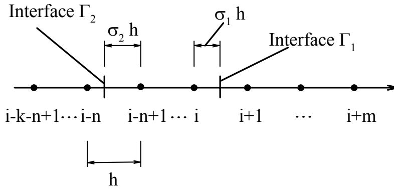
Fig. 5. Uniform grid with two interfaces surrounding an irregular point i .
