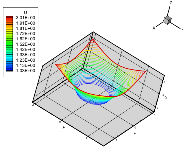
Fig. 11. Solution, z = u(x, y) , computed by Method A ( O(h^2) ) for the first two-dimensional example.
