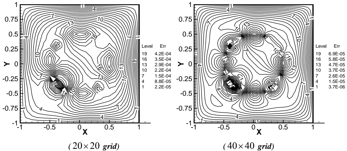
Fig. 18. Contours of local errors computed by current second-order interface method A for two sets of grids.
