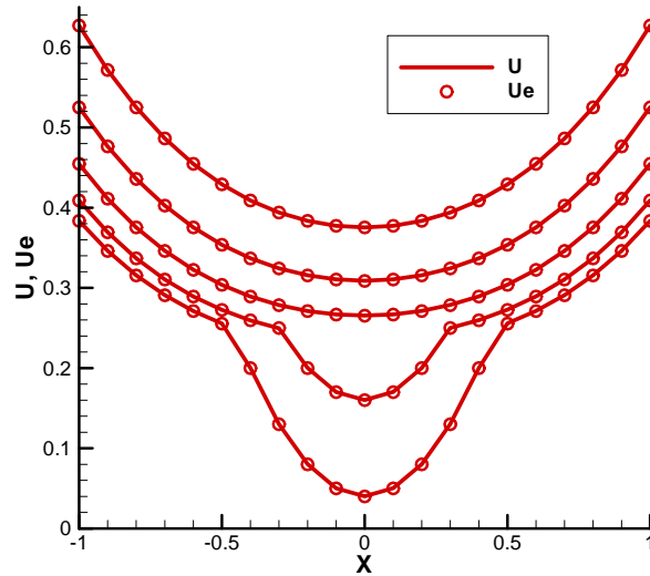
Fig. 17. Comparison of the profiles of the exact ( u_e ) and numerical ( u ) solutions along a number of horizontal grid lines. The numerical solution is computed by Method A with a set of 20 \times 20 grid.
