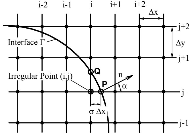
Fig. 10. A schematic of a two-dimensional uniform grid with an immersed interface \Gamma , where (i, j) is an I-directional irregular point (J-directional irregular points can be defined similarly).
