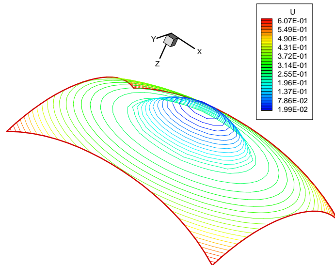
Fig. 16. Solution, z = u(x, y) , computed by Method A ( O(h^2) ) for the second two-dimensional example with a set of 20 \times 20 grid.
