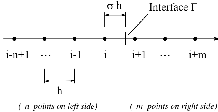
Fig. 2. Uniform grid with an interface located on the right side of irregular point i with a general grid stencil of n and m points on the left and right sides, respectively.
