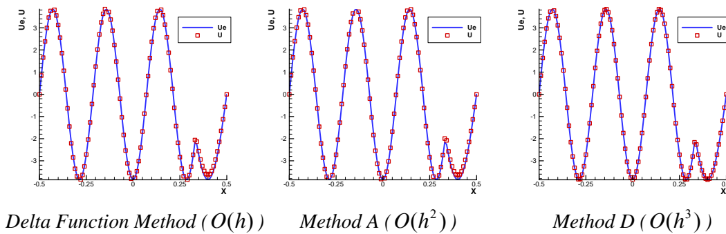
Fig. 8. Comparison of the exact and numerical solutions for computing one-dimensional equation with a discontinuous coefficient and a singular source term ( N = 80 ).
