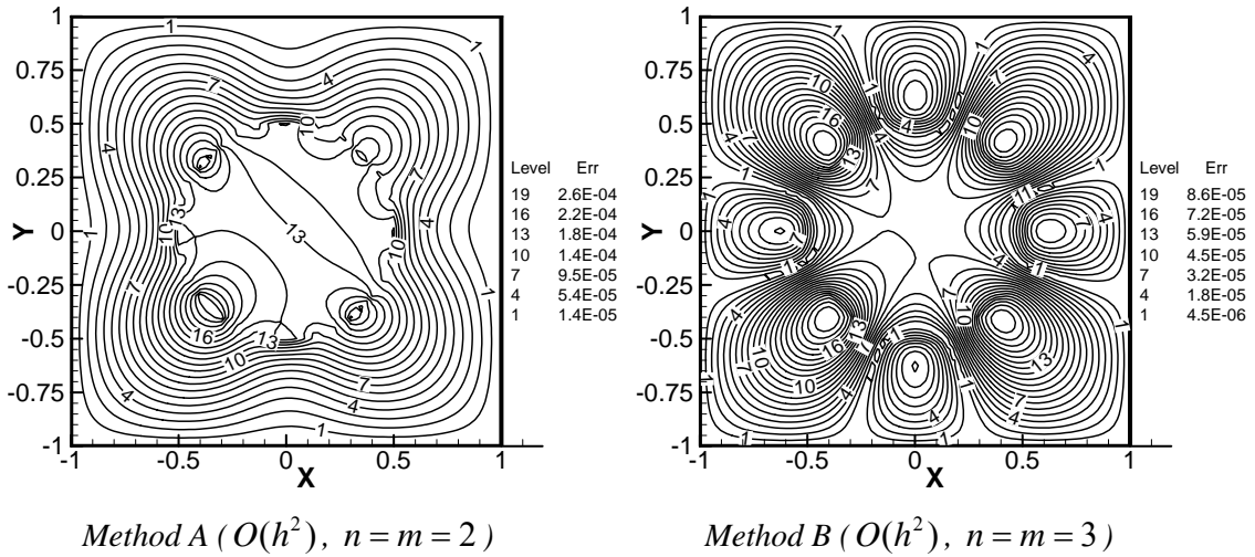
Fig. 14. Contours of local errors computed by two current interface methods. Both methods use the same O(h^2) approximation at regular points, but their irregular point treatments are of different orders, ranging from O(h) to O(h^2) (grid: 80 \times 80 ).
