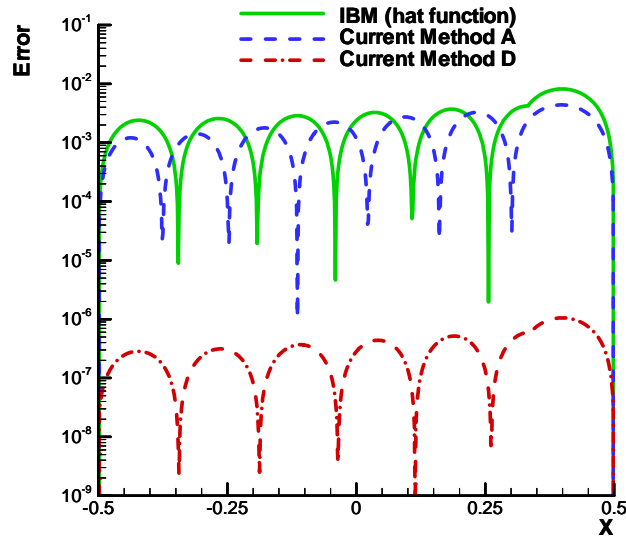
Fig. 9. Comparison of numerical errors for solutions computed by three numerical methods ( N = 640 ).
