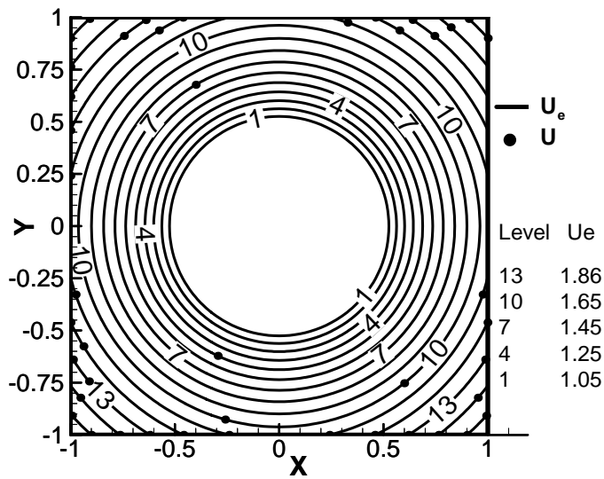
Fig. 12. Comparison of the contours of the exact ( u_e ) and numerical ( u ) solutions. The numerical solution is computed by the current Method E ( O(h^4) , irregular points: n = m = 4 , grid: 80 \times 80 ).
